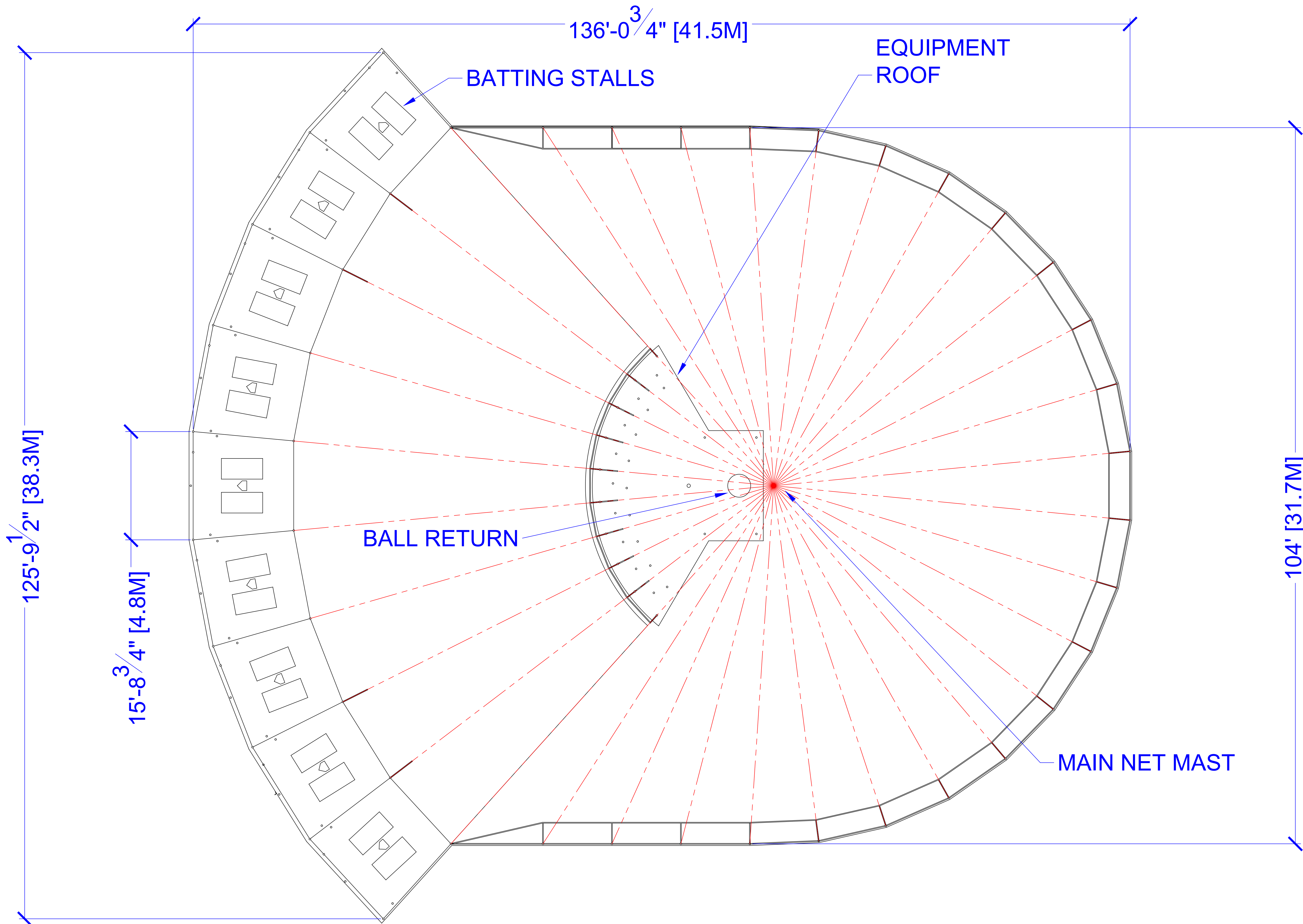
STANDARD OUTDOOR 9 CAGE SYSTEM
